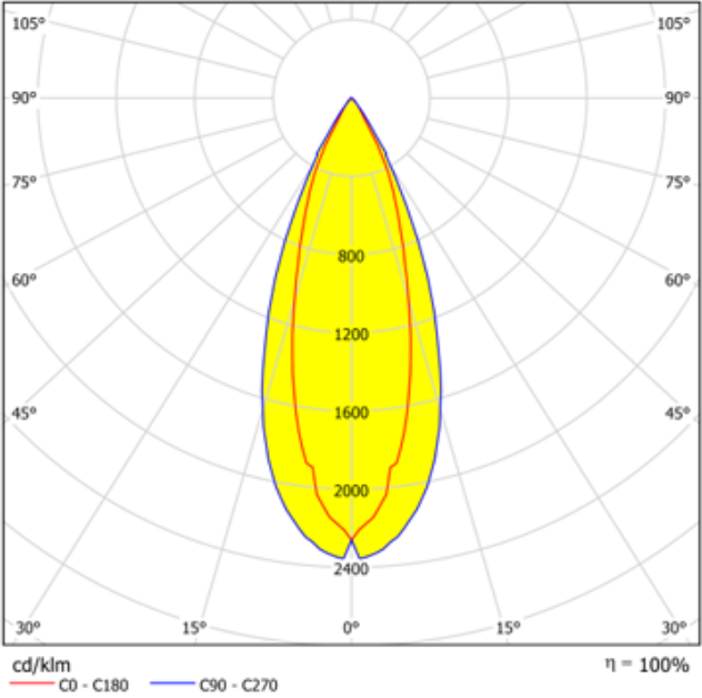
20°/45° Black Baffle Glare
